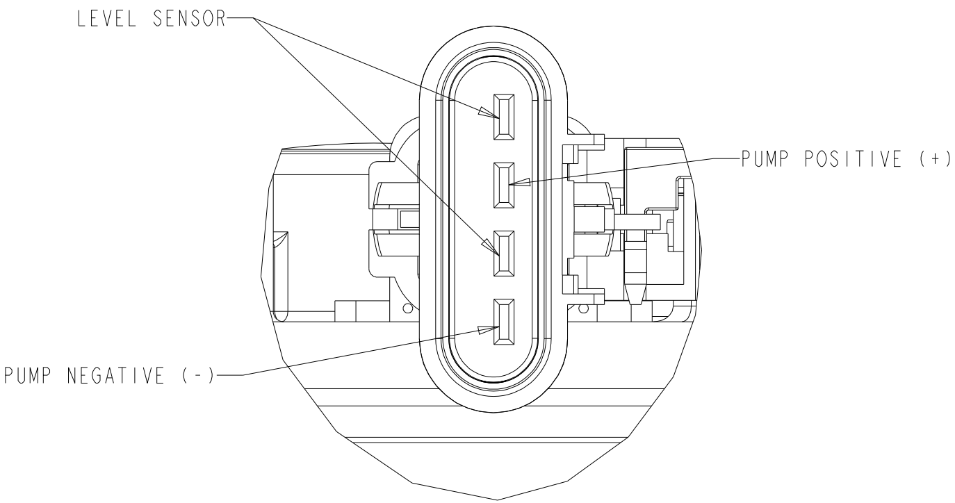
VIEW X SCALE 2:1
